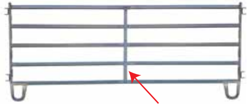
Panel comes standard without the center strap & does not come installed. 12' PANEL WITH LOOP FEET STANDARD OVAL 5 RAILS, ROUND END POSTS, OPTIONAL CENTER BAR
