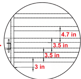
Panel Spacing (Bottom Rails)
