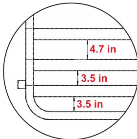
Gate Spacing (Bottom Rails)
