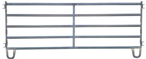
12' PANEL WITH LOOP FEET STANDARD OVAL 5 RAILS, ROUND END POSTS
