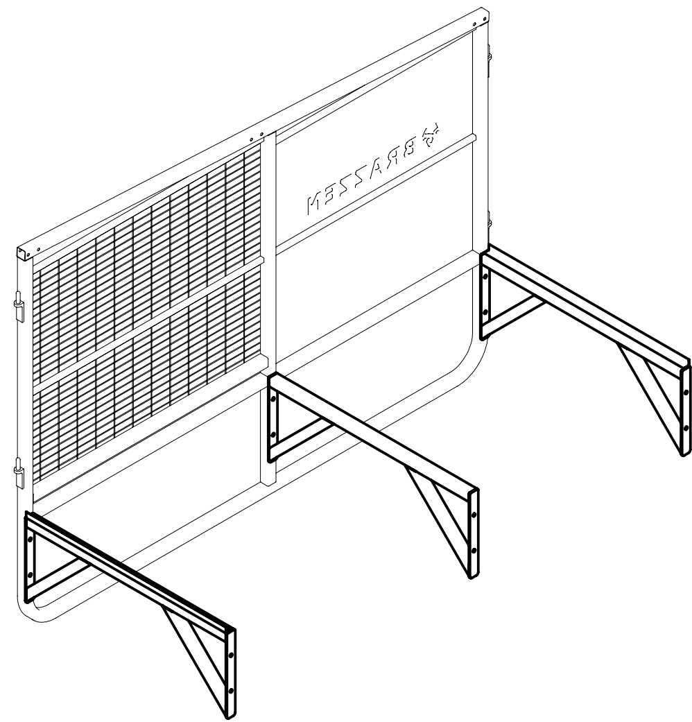
+6-BOLT/M10x60 & NUT/M10
