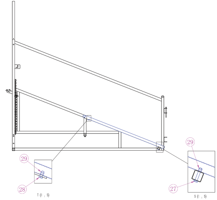
Sheep Loading Ramp Walkway Kit complete
